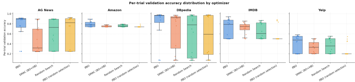
Figure 7: Per-trial accuracy distribution.
