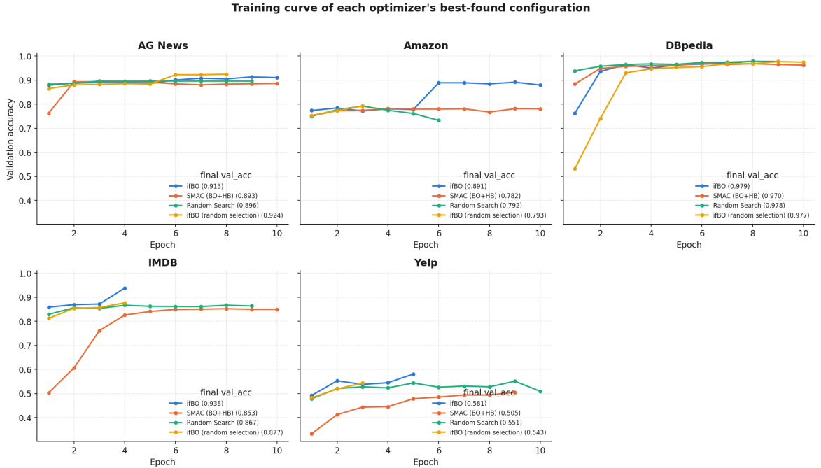
Figure 9: Best trial training curves per dataset.
