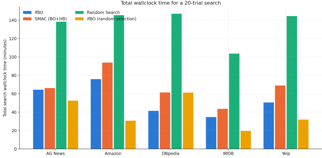
Figure 6: Total wall-clock time per dataset and method.
