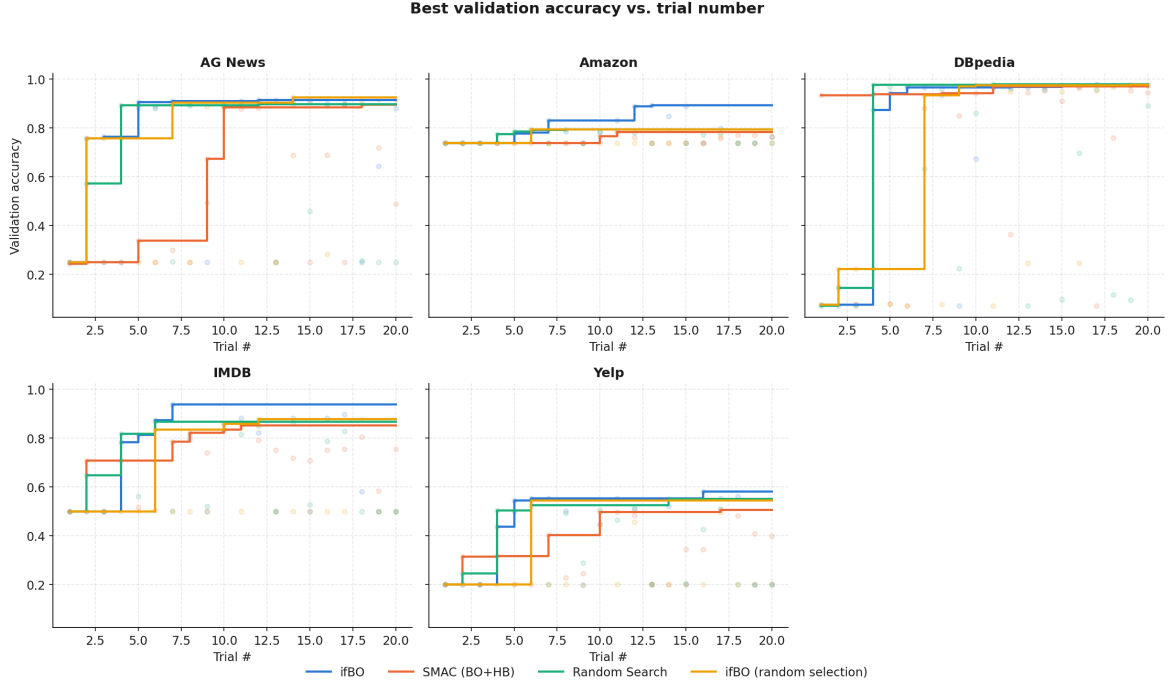
Figure 4: Best validation accuracy vs. trial number.
