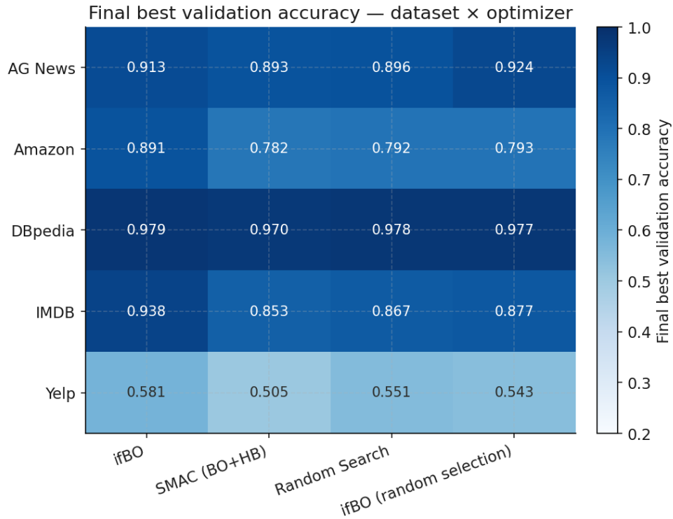
Figure 3: Accuracy heatmap across datasets and methods.
