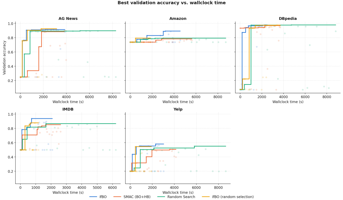
Figure 5: Best validation accuracy vs. wall-clock time.
