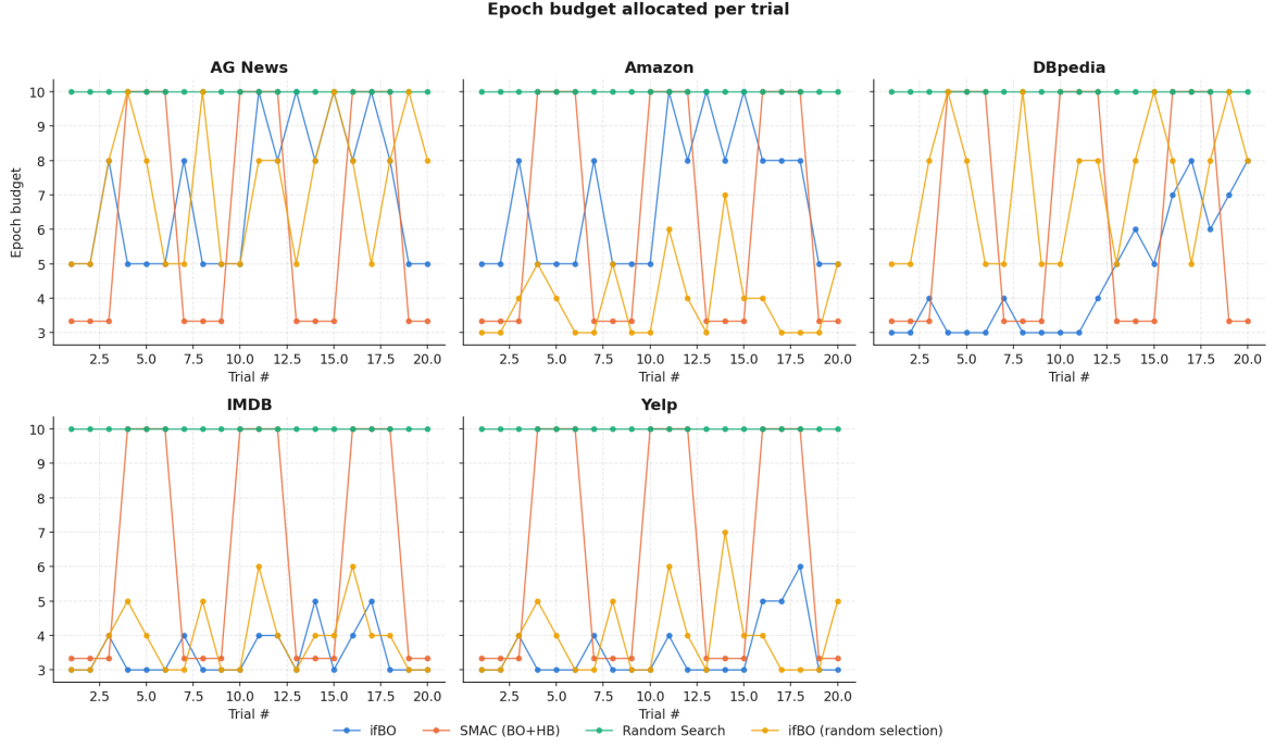
Figure 8: Epoch budget allocated per trial.
